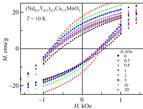
FIG. 3. Magnetic hysteresis loops for (\text{Nd}_{0.9}\text{Y}_{0.1})_{2/3}\text{Ca}_{1/3}\text{MnO}_3 obtained at 10 K after cooling in a magnetic field H_{\text{cool}} = 0.5, 0.8, 1, 2, 5, 10 , and 20 kOe.
